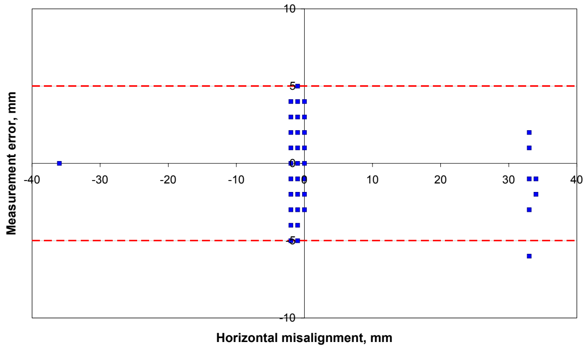
Figure 30. Measurement error on vertical misalignment as a function of horizontal misalignment (MIT test track).
