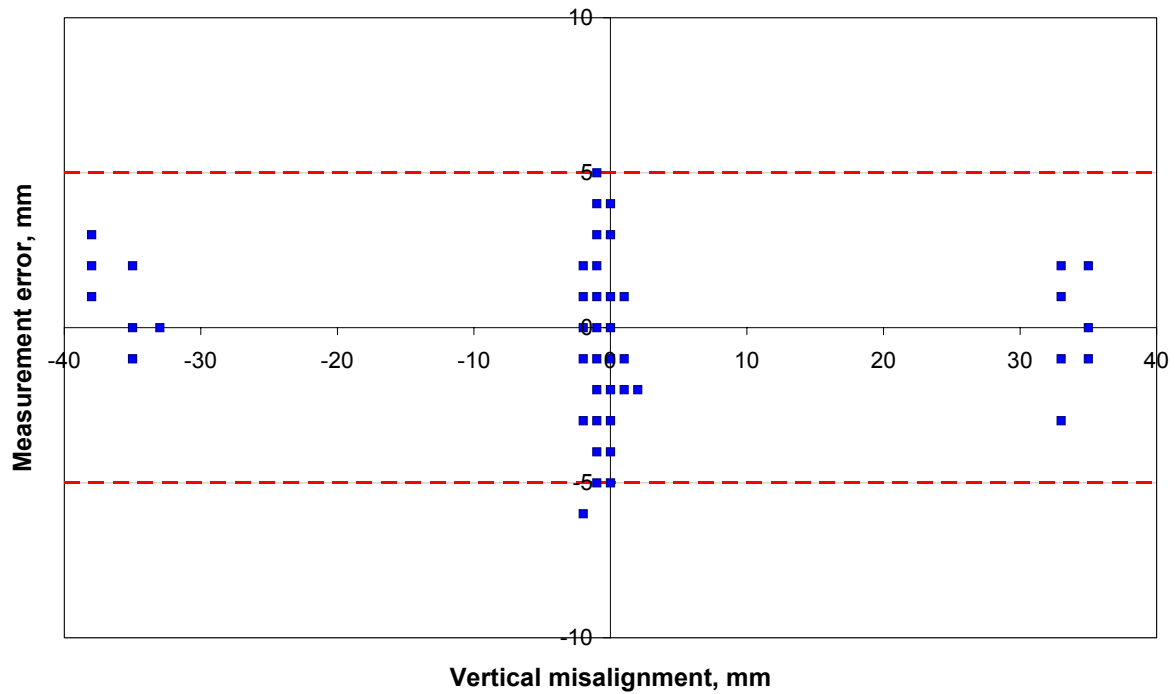
Figure 32. Measurement error on vertical misalignment as a function of vertical misalignment (MIT test track).
