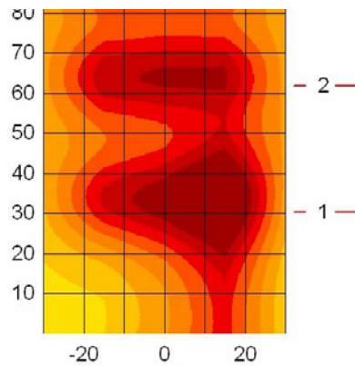
Figure 23. Presence of tie bar directly over the outer dowel bars.
